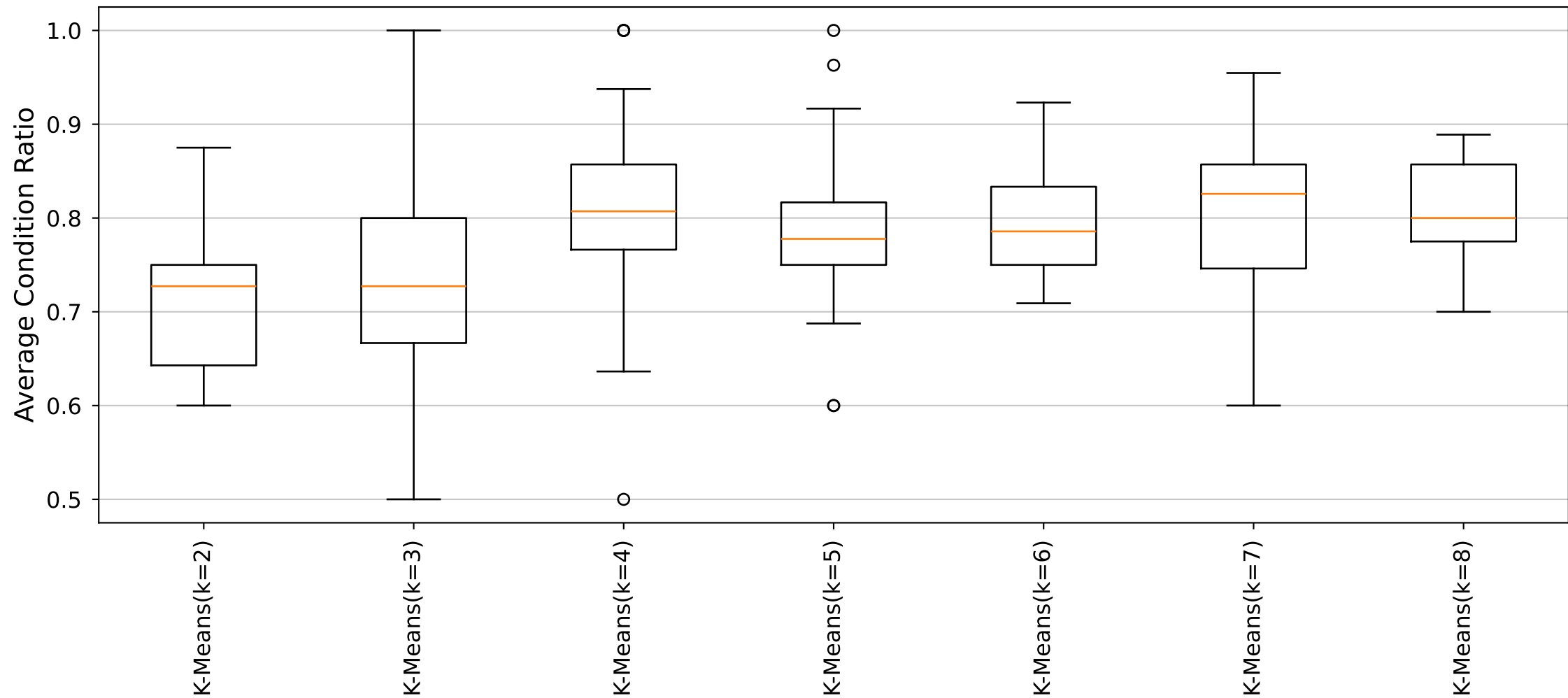
YARA Rules Average Condition Ratio Distribution (Cluster17_Size8 dataset)
